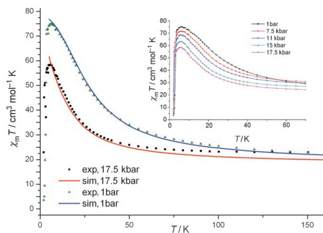
Figure 3: Plots of \chi_M T versus T for 1 recorded in the temperature range 150–5 K and 60–5 K (inset) shown at the indicated pressures. The solid lines represent simulations of the data; see text for details.
